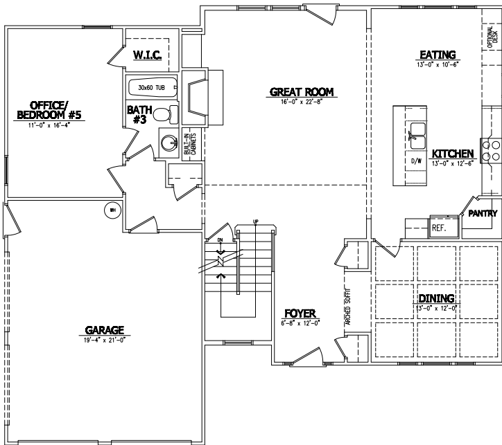
Main Level
